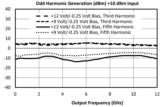
Typical Performance – +9 to +12V Internal Bias (Pin 11), -0.25 Negative Bias (Pin 6), continued
